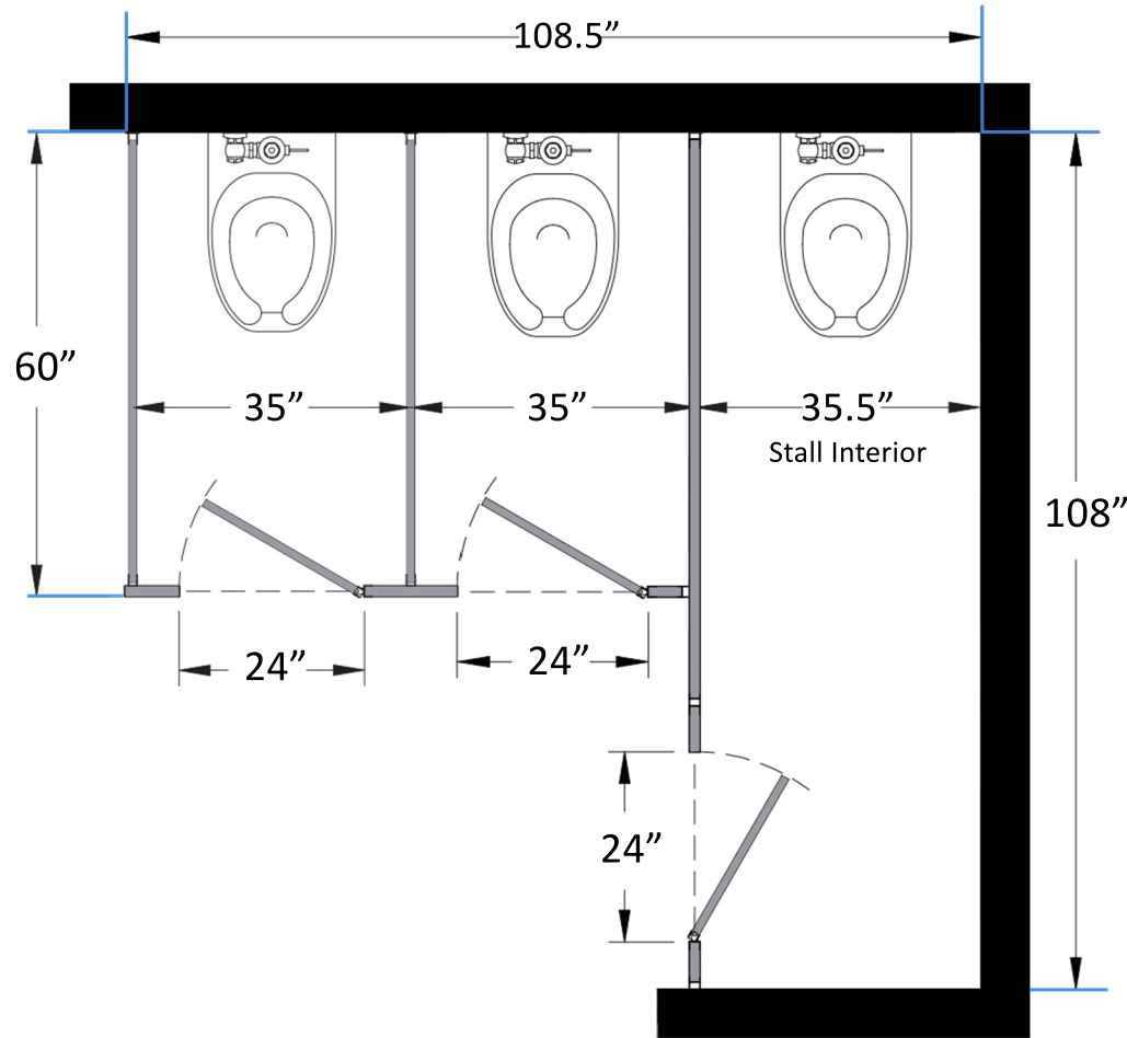
Bathroom Partitions - 3 Stall Alcove Right Hand SKU: ALIC3R Standard Dimensions
